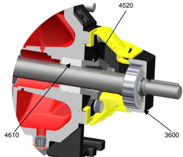
Stuffing box
